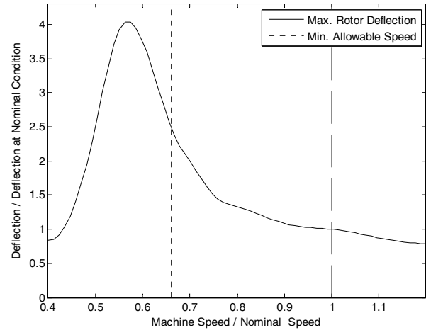
Figure 2: Rotor Deflection vs. Machine Speed for Centrifugal Compressor Rotor.
