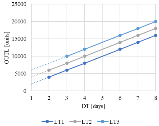
Figure 3 – Scenario 1; trend of the optimal combinations of the operating leverages DT and Outil
