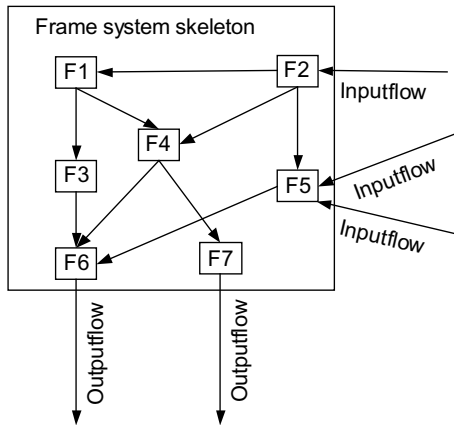
Figure 4: Frame Model representing the agent architecture
