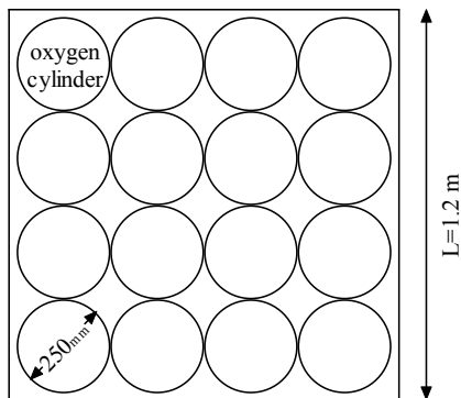
Fig. 5 – Light metal alloy load unit
