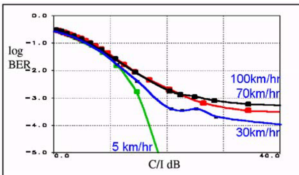
Figures 9b: OmniSys simulation of BER vs. C/I in NADC (IS-54) flat fading channel for different mobile speeds.
