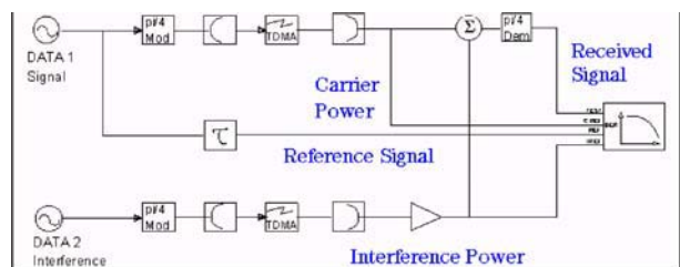
Figures 9a: An OmniSys simulation of an IS-54 system including fading radio channel with CCI.
