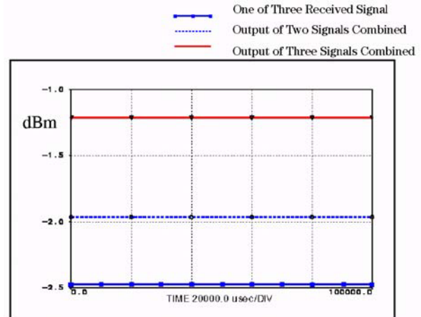
Figures 8d: Average power.
