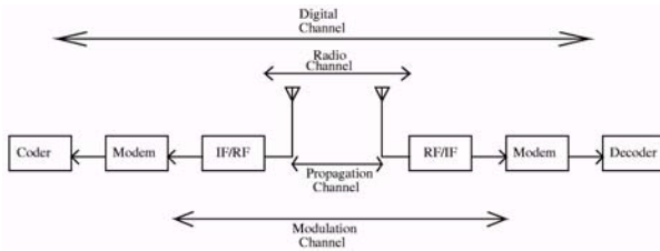
Figures 1: Various channels in a communications system.
