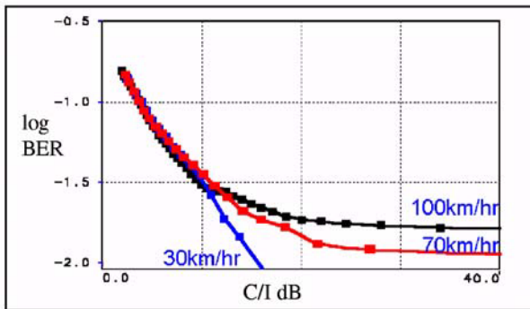
Figures 10b: BER vs. C/I in GSM propagation channel for different mobile speeds.
