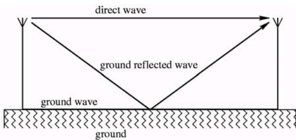
Figures 2: The two ray, flat earth model.
