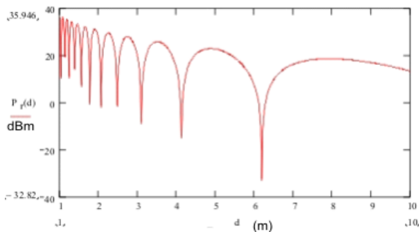
Figures 3: Losses of capacity of a signal in a point of reception P_r(d) (dBm) as function from distance d (m).
