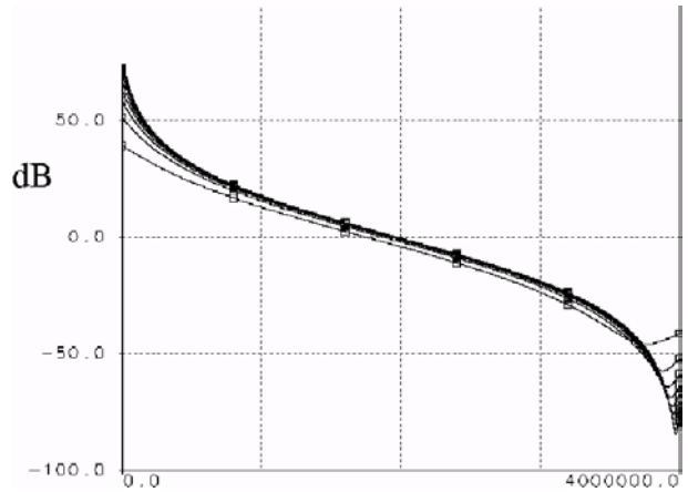
Figures 7b: C/I ratio as a function of time or distance.
