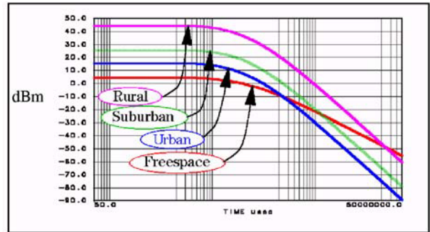
Figures 4: Comparison of Hata's pathloss models for different environments.
