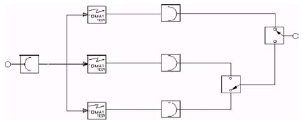
Figures 8a: Switched combining scheme for reducing the fade margin.
