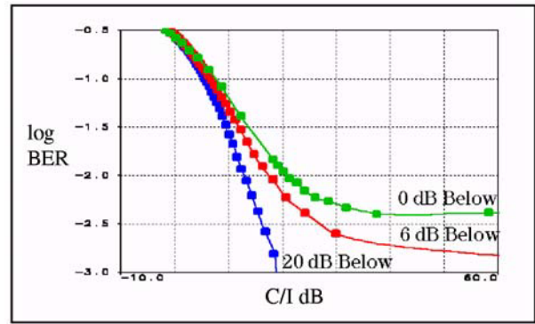
Figures 9c: OmniSys simulation of BER vs. C/I for different ratios of 1st over 2nd ray powers.
