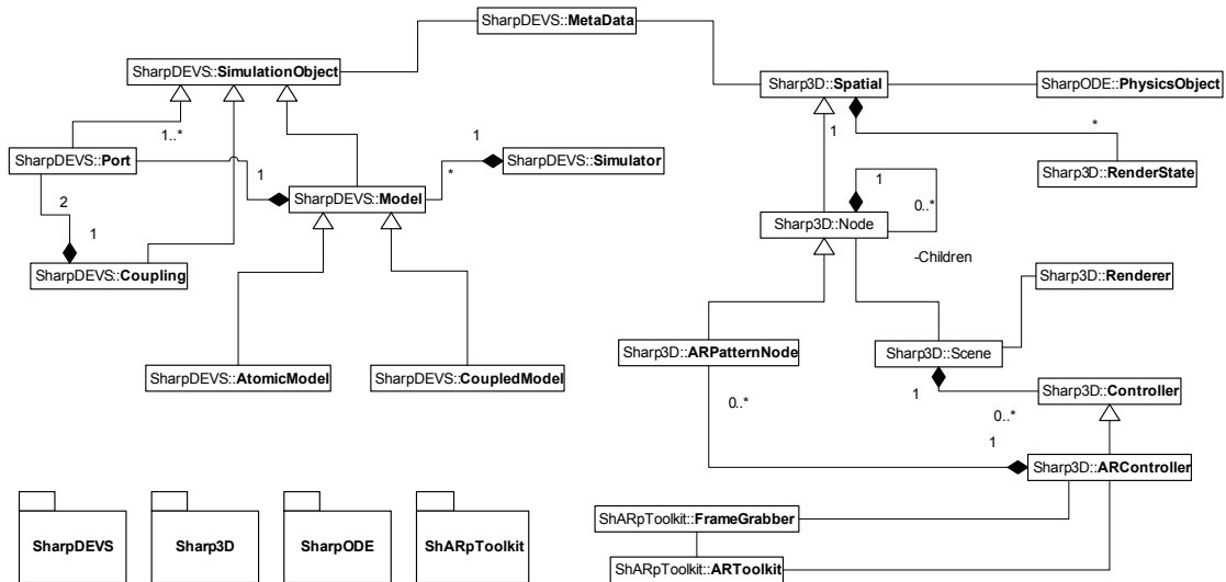
Figure 7: Generalized SharpSim Class Structure Diagram
