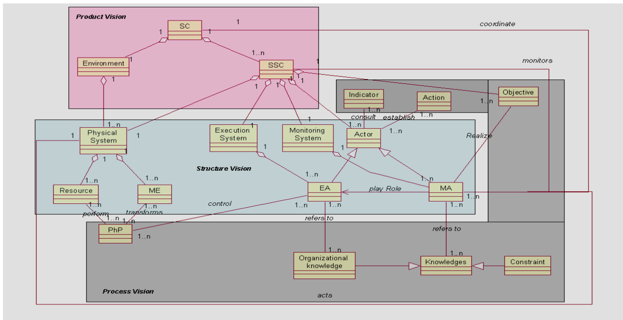
Figure 3. Domain metamodel
