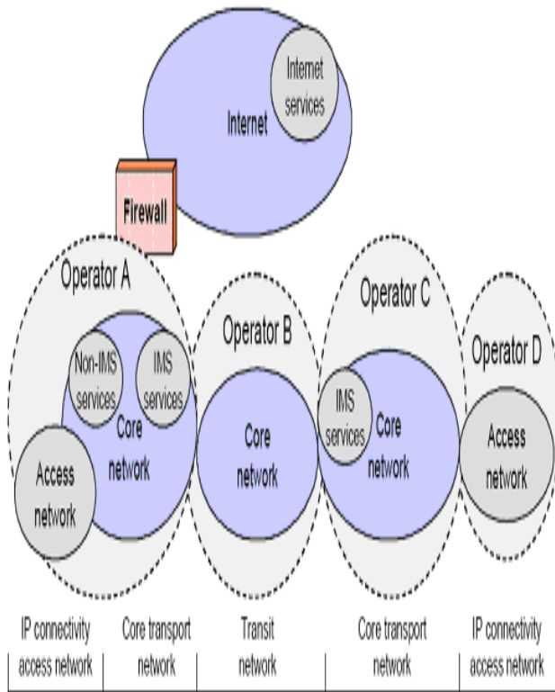
Figure 6. Network Partition on the basis of IMS Source: VTT, Technical Research Centre of Finland (2007).
