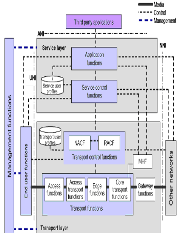
Figure 5. Overview of NGN Functional Architecture
