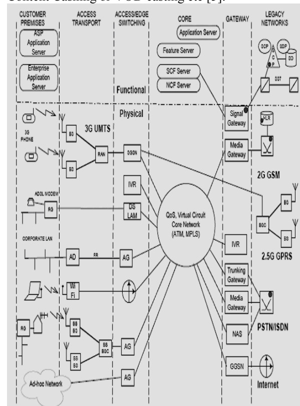
Figure 9. Heterogeneity environment of NGN and relation with legacy network
