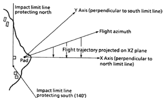
Figure 1 Impact limit line
