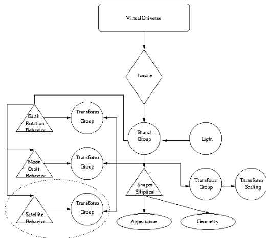
Figure 7 Scene graph for planetary and satellite orbit
