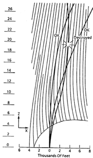
Figure 3 Vertical plane destruct line
