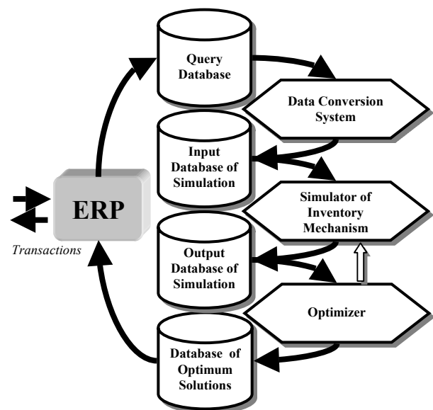
Figure 1. Process of the dynamic inventory management
