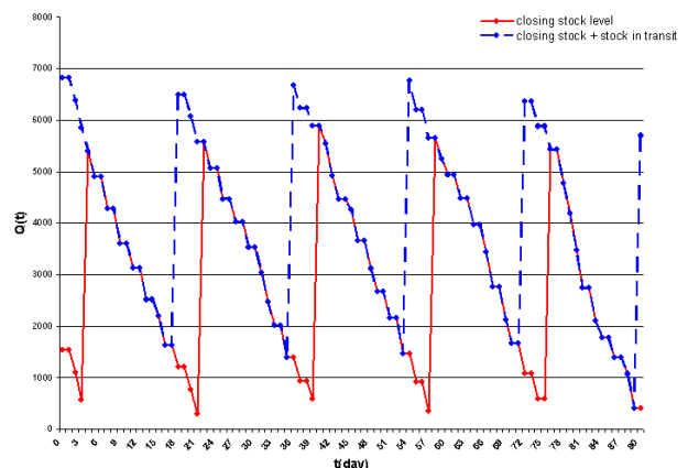
Figure 2. Operation of the [t;q] mechanism (stock levels)
