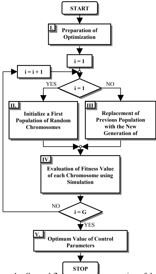
Figure 4. General flowchart of the operation of the binary genetic optimizer
